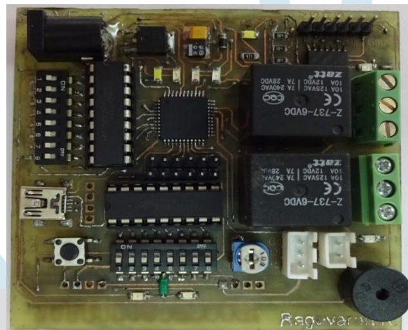
Fig. 6. Top side of slave-1 hardware
