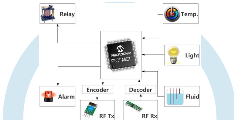
Fig. 3. Block diagram of Slave-1 module.
