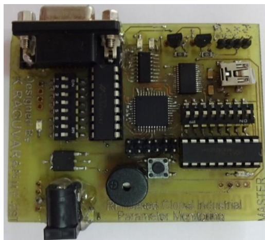
Fig. 5. Top side of master hardware
