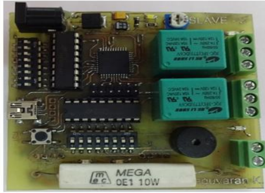
Fig. 7. Top side of slave-2 hardware
