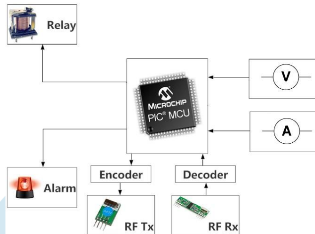
Fig. 4. Block diagram of Slave-2 module.
