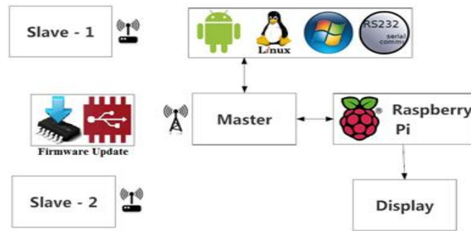
Fig. 1. Block diagram of the process monitoring system using Raspberry pi.
