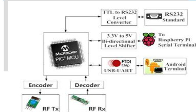
Fig. 2. Block diagram of master module.
