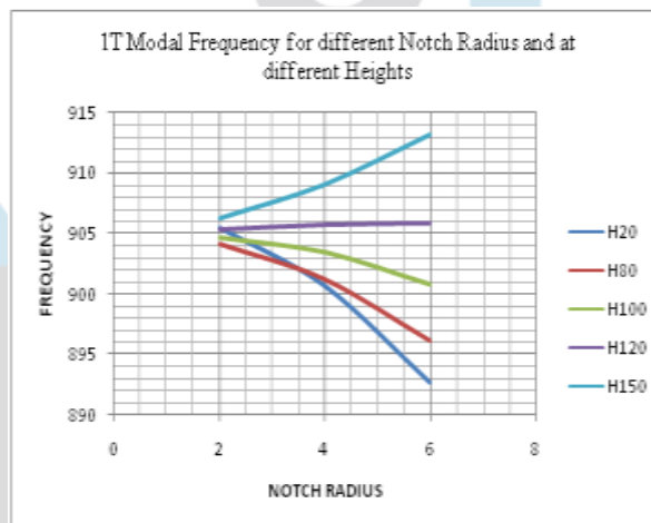
Graph 2: 1t Modal Frequency Vs Notch Radius
