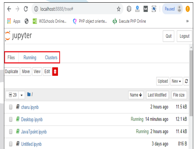
Fig.9 Jupyter Notebook
