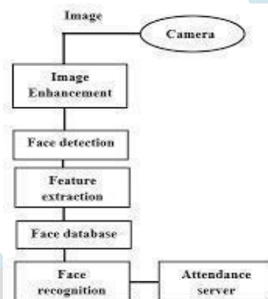
Fig-1: A structure diagram that shows how faces are detected.
