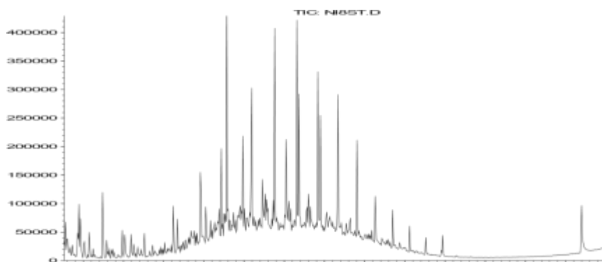
Figure 4. 5. Typical GC-MS chromatograms of (a) transformer oil (tridecane to docosane), (b) shale oil (decane to phytane), and (c) diesel fuel (octane to octacosane) with an internal standard at 28.8 min.
