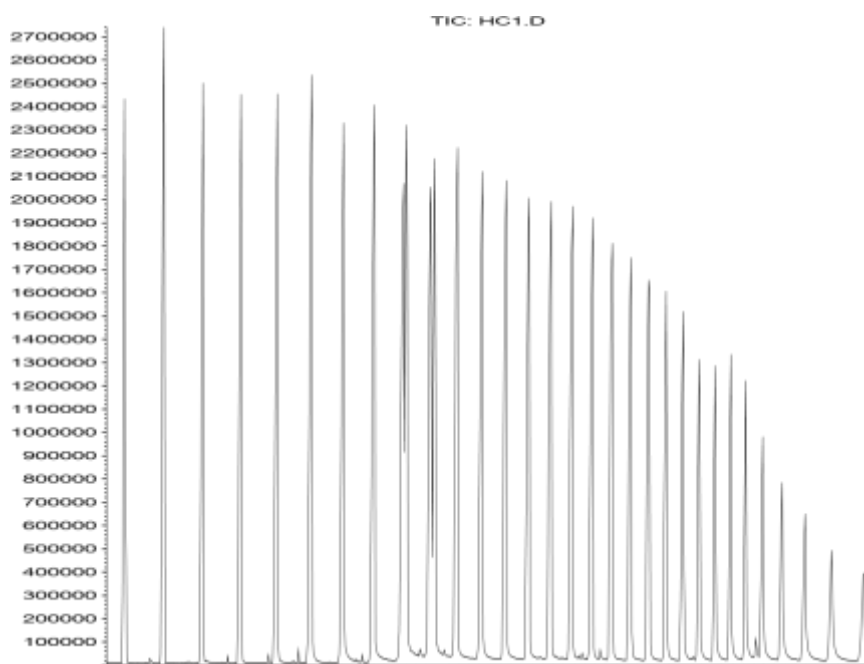
Figure 4. 4. Displays the GC-MS output for a standard mixture of hydrocarbons, used here to establish the detection limits and calibration range for DRX window analysis.
