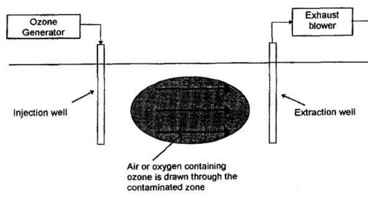
Figure 3. 3. presents a layout of an ozone injection system designed for in situ treatment of polluted soil environments
