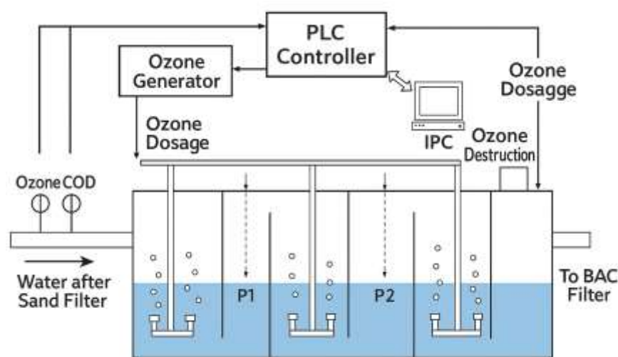
Figure 3.2: Schematic of Equipment Used for Ozonation
