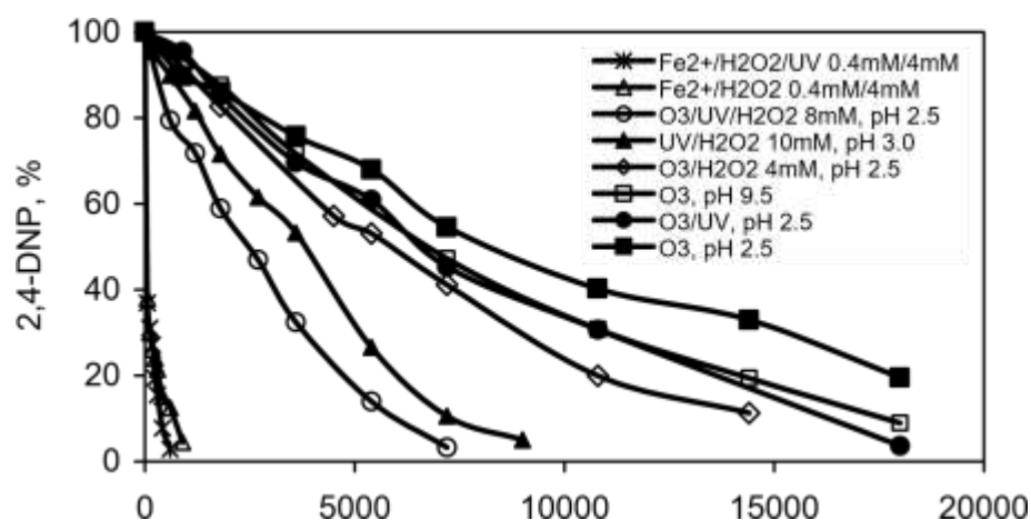
Figure 5. 1. 2,4-DNP Degradation under Various Treatment Methods
