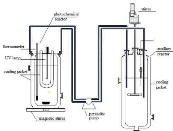
Figure 4. 1. Schematic diagram of the experimental setup used for UV/ \text{H}_2\text{O}_2 oxidation.
