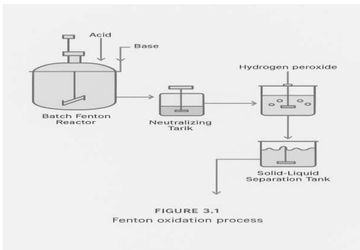
Figure 3.1. Scheme of the Fenton oxidation treatment
