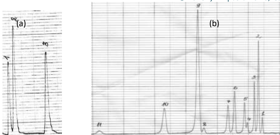
Figure 4. 3. Typical chromatograms of (a) nitrophenols obtained by HPLC-UV detection at 280nm: (1) 4-nitrophenol; (2) 2,4-dinitrophenol; (3) 4,6-dinitro-o-cresol; and (b) polycyclic aromatic hydrocarbons with fluorescence detection at 254 nm
